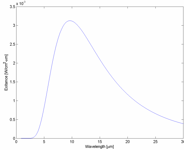
Figure 3. Radiant Exitance for a Blackbody at 300K (7)
