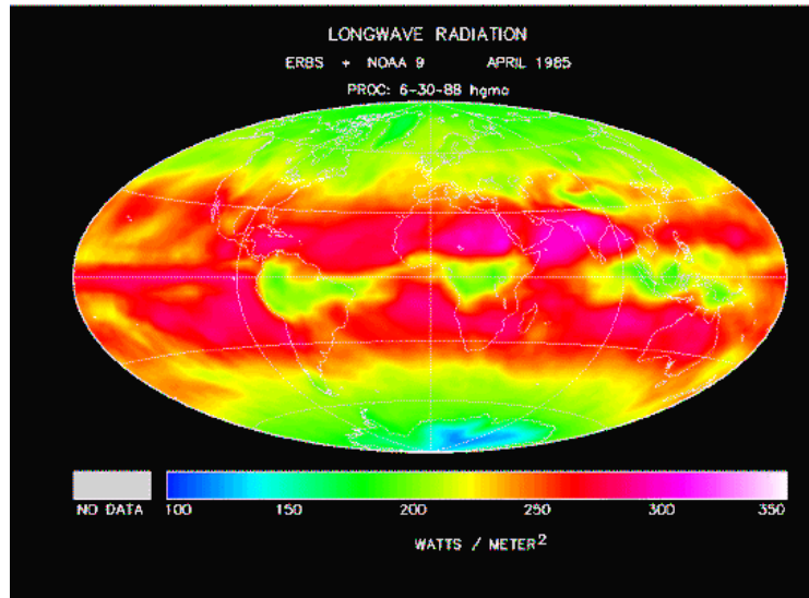
Figure 5. Intensity Map of Top-of-Atmosphere Emitted Longwave Radiation
