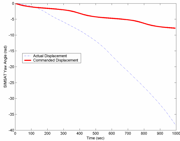
Figure 17. Initial Measurements of SIMSAT Body Yaw Rate with Forced \dot{\mathbf{b}}
